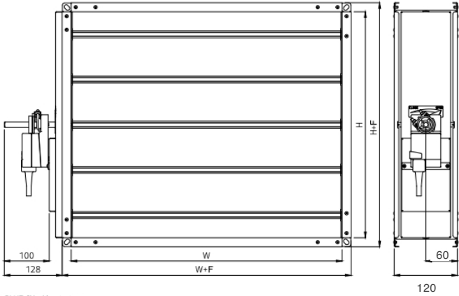
BLUE-SX with actuator
